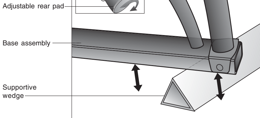
Diagram 9 Place the base on supportive blocks.
